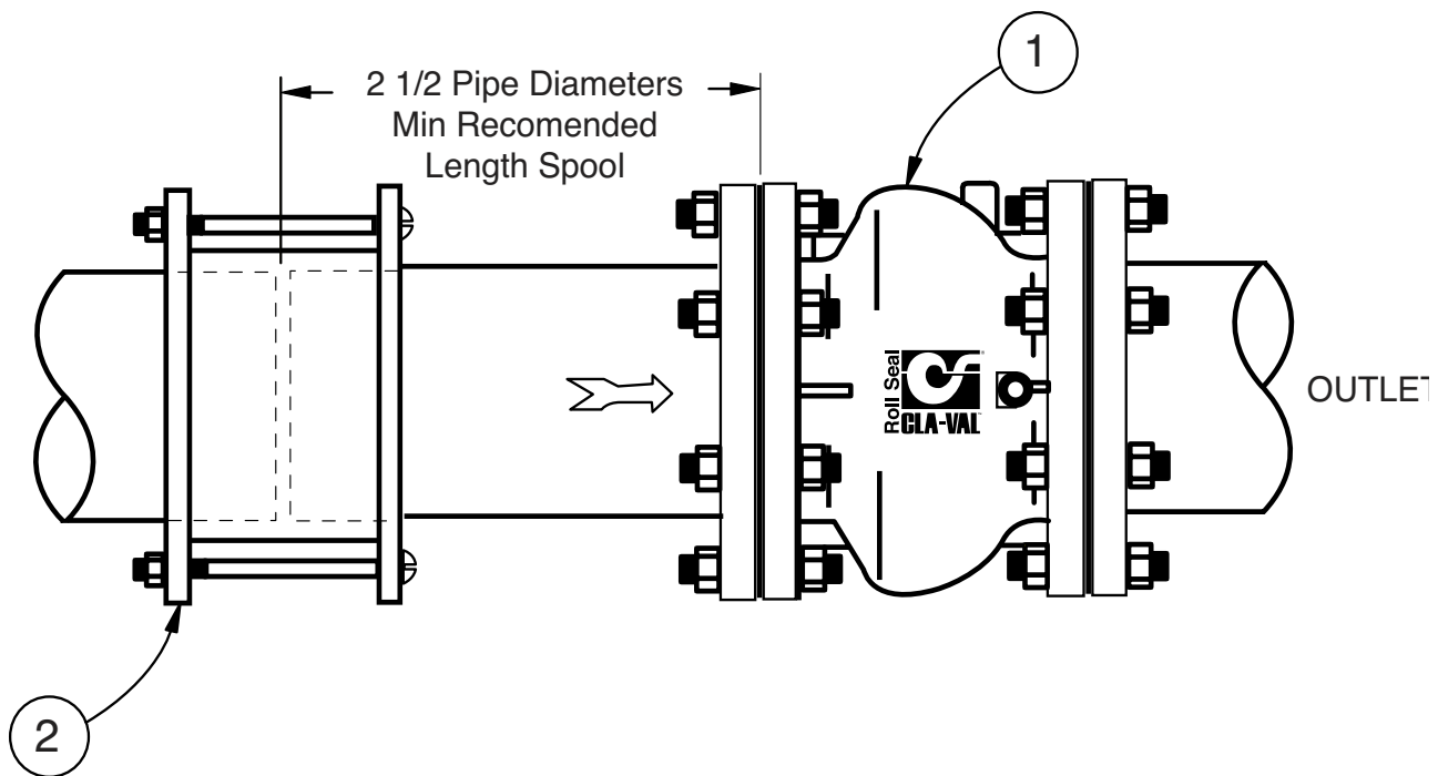
Recommended Pipe layout 6" - 12" Flange style 100-42
