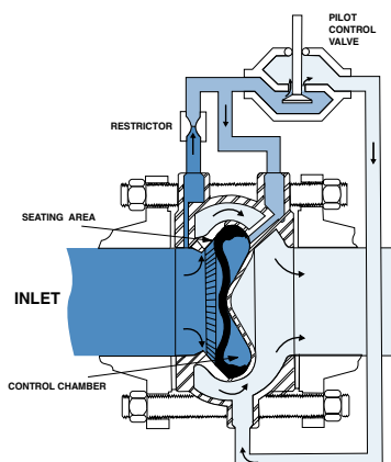
Model 100-42 Valve in Partially Open Position
