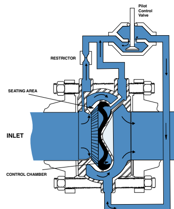
Model 100-42 Valve in Fully Open Position
