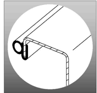
Fig. 3-6: A side sealing can be fastened to the returned edge of the side wall.
