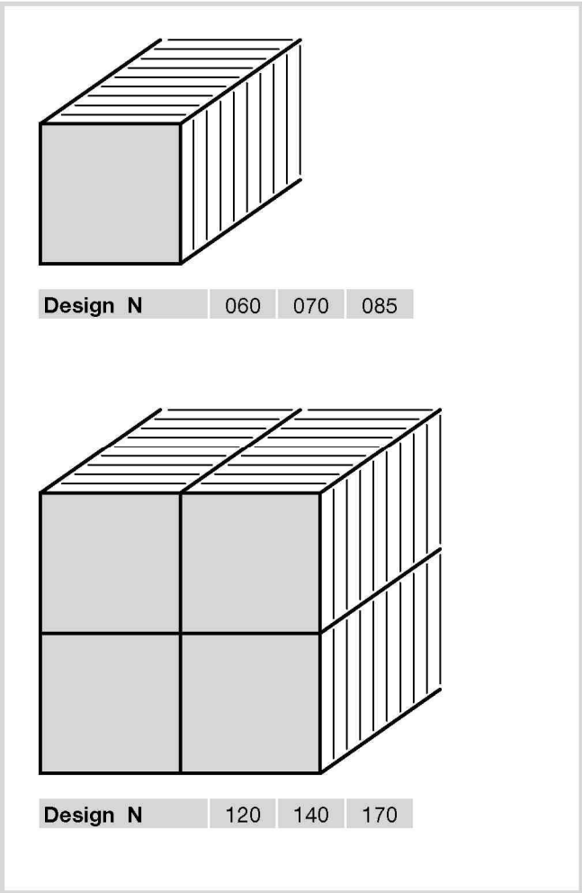
Fig. 4-2: Individual plate heat exchangers are constructed from different exchanger packages.
